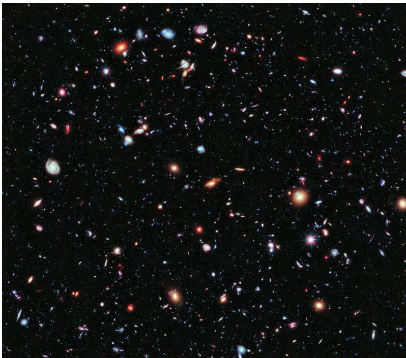
Galaxies in the Hubble Extreme Deep Field. Every smudge in the image is a distant galaxy.
