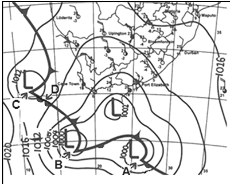
FIGURE 1.3: MID-LATITUDE CYCLONES
