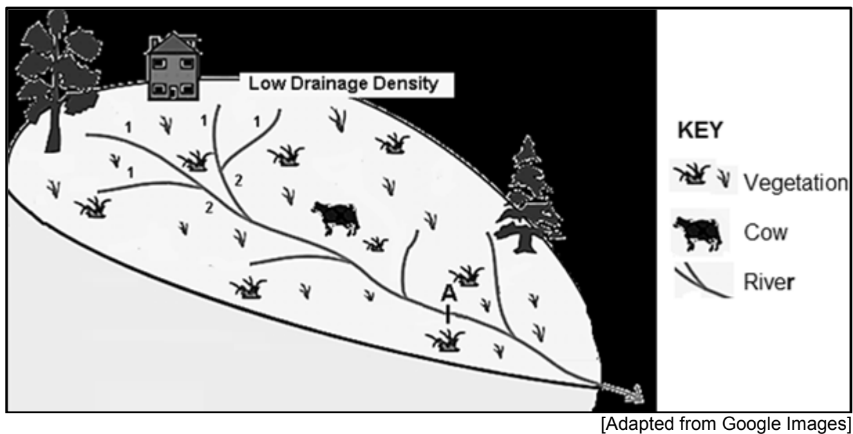
FIGURE 1.5: DRAINAGE DENSITY
