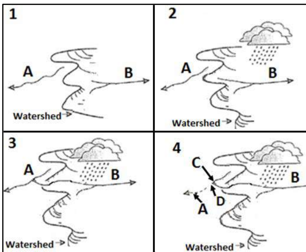
FIGURE 1.2: RIVER CAPTURE
